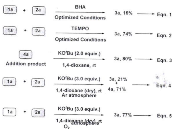
Scheme 4: Control Experiments
