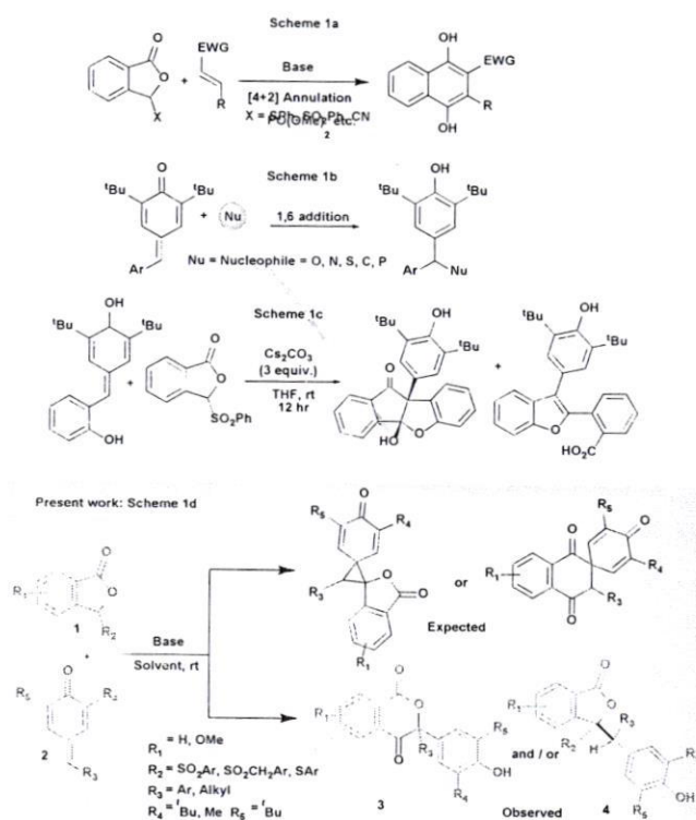
Scheme 1: Synthetic approaches to SP and p -QMs
